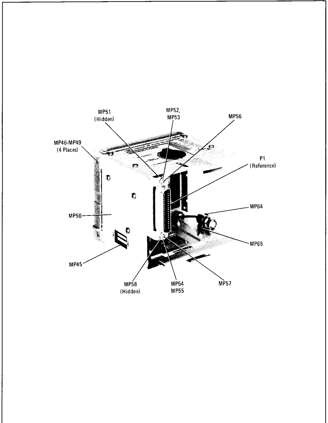
Figure 6-1. Mechanical Parts (1 of 2)
